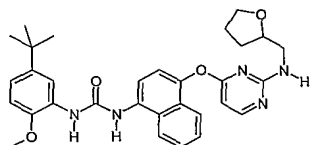
1-(5-tert-Butyl-2-methoxy-phenyl)-3-(4-{2-[(tetrahydro-furan-2-ylmethyl)-amino]-pyrimidin-4-yloxy}-naphthalen-1-yl)-urea;
